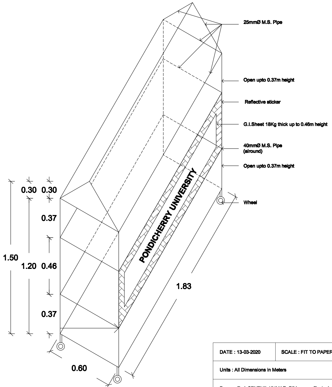
1. Barricade Sectional cum Elevation (Wheel type requirements - 10 Nos)
